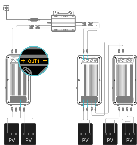
Diagram for Connecting 3 B2500-D
