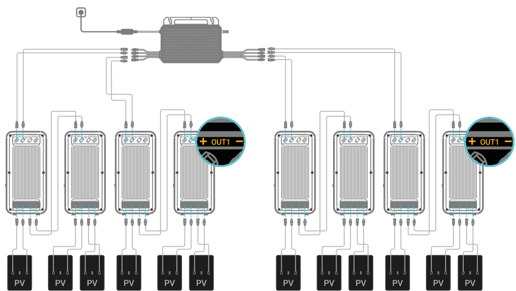
Micro Inverter with Four MPPT
