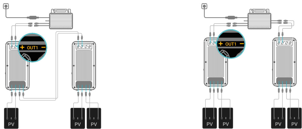
Diagram for Connecting 2 B2500-D
